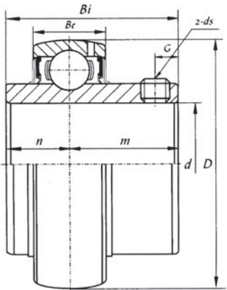
UC 300 (heavy-duty)
