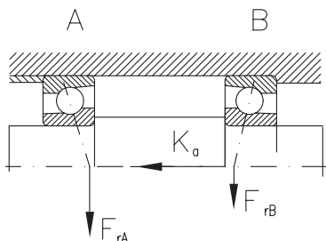
Face to face arrangement DF
