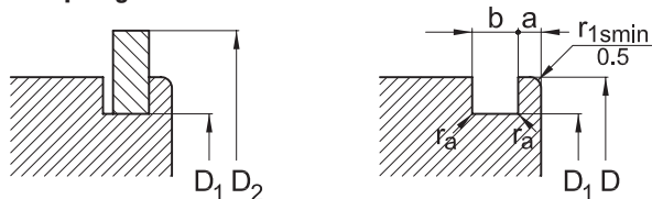
Snap ring groove
