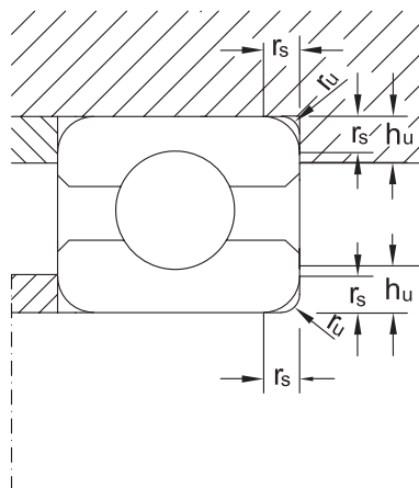
Abutment dimensions
