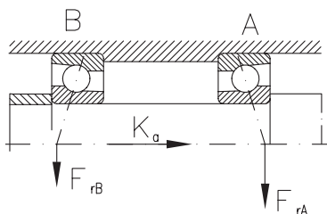
Back to back arrangement DB
