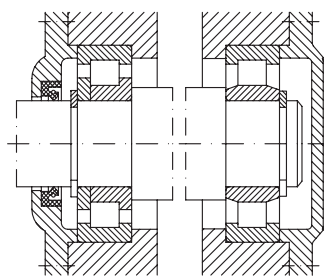
locating bearing d) non-locating bearing
