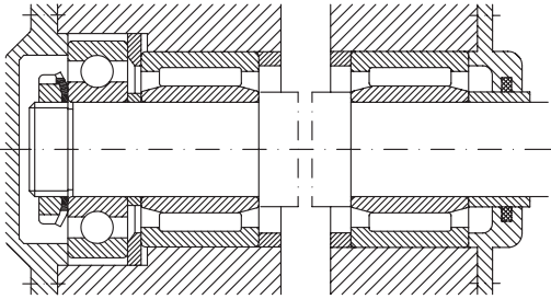
locating bearing f) non-locating bearing
