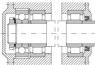
locating bearing e) non-locating bearing
